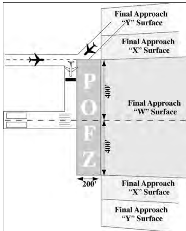
NEW FIG 3-7-1 Precision Obstacle Free Zone (POFZ)
